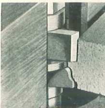
Making a combination rabbet and ogee cut on sash stock, using a spacing collar between cutters.
